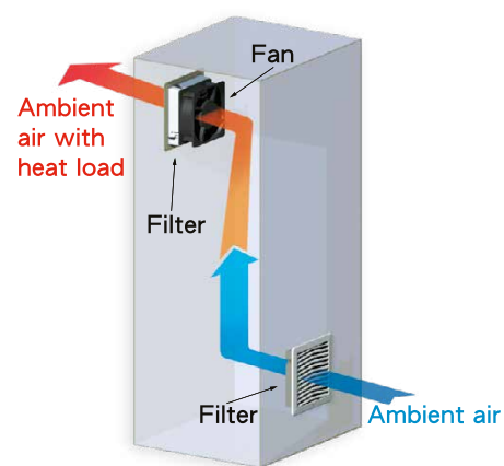
Fig.1 Exhaust system
